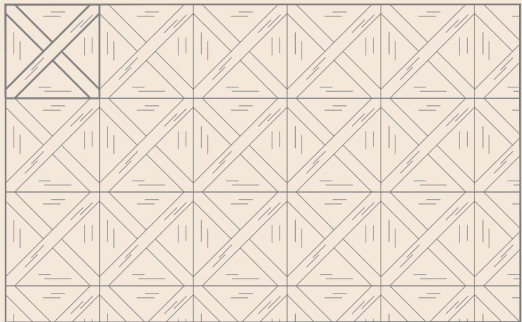
Mogliano 590x590mm 2 strati / 2 layers sp. / th. 16mm - 14mm
