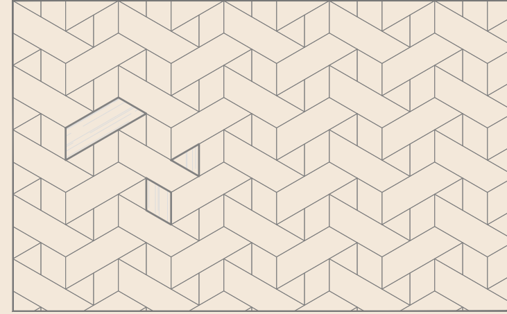
Nisia - Posa / Installation 430 600x180mm, 208x180mm, 208x160mm
