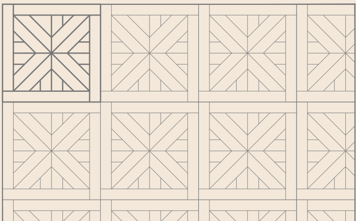
Sanremo 900x900m 2 strati / 2 layers sp. / th. 16mm
