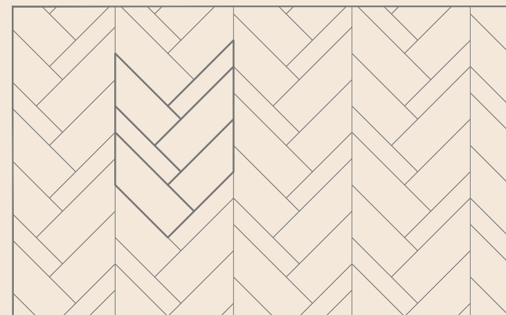
Soul - Posa / Installation 410 720x240mm, 600x240mm, 600x120mm, 120x120mm
